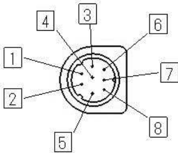
miniDIN 8pin
